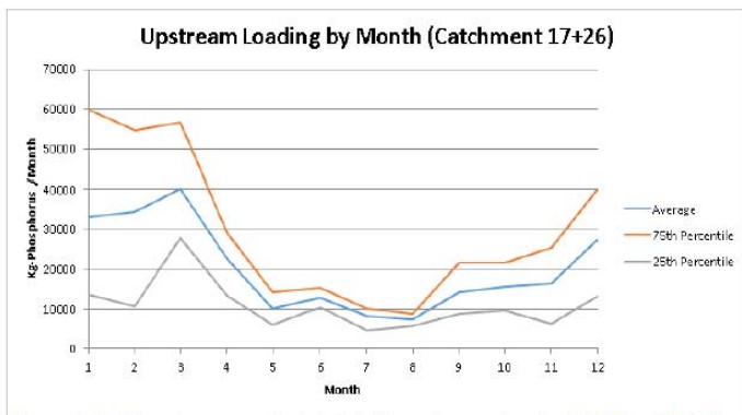
Figure 7-2 Upstream routed total phosphorus loads (2008 – 2013)
