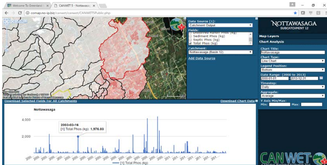
CANWET-5 Nottawasaga River Platform: Historical Phosphorus Loads from Priority Subwatersheds (2017)
